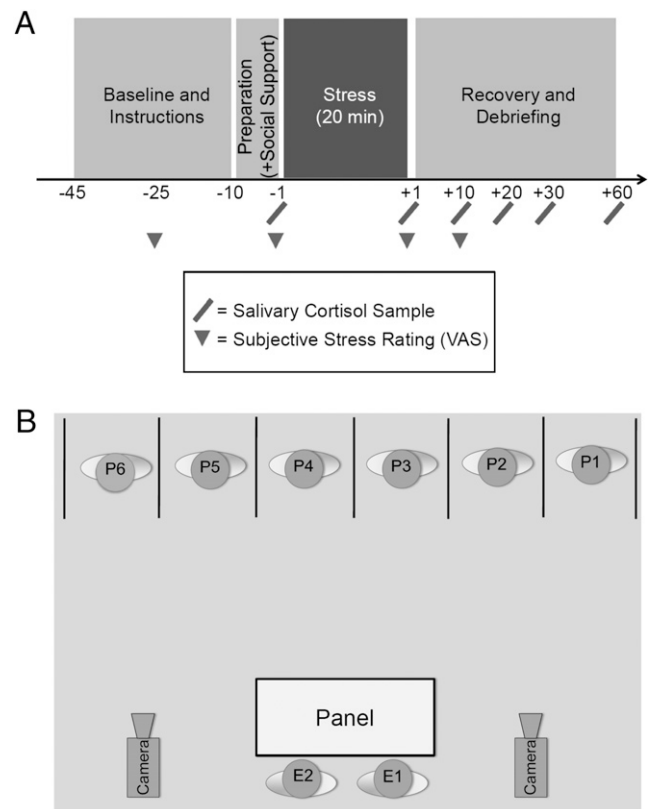
Fig. 3. (A) Sequence of events and timeline of the study protocol. (B) Layout of stress room, depicting six participants (P) and two evaluators (E). VAS, visual analog scale.
